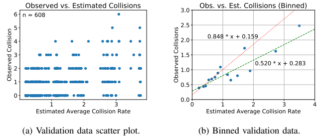
Fig. 8: Results from validation scenes for the ReSonAte framework. Each data point shown in Fig. 8a represents the outcome of one simulated scene with the actual number of collisions observed plotted against the estimated average collision rate. These same data points have been divided into bins and averaged in Fig. 8b, along with two least-squares fit trend lines.
